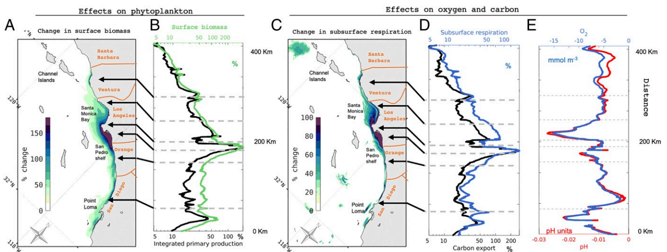
Fig. 3. Biogeochemical effects of land-based and atmospheric nitrogen inputs in the SCB. (A) Surface chlorophyll enhancement (%) in the ANTH simulation, relative to the CTRL simulation. (B) Alongshore surface chlorophyll (green line) and vertically integrated net primary production (0 to 80 m, black line) enhancement (%). (C) Subsurface (40 to 80 m) respiration enhancement (%). (D) Alongshore subsurface (40 to 80 m) respiration and carbon export enhancement (%). (E) Absolute alongshore O 2 ( \text{mmol m}^{-3} ; blue line) and pH (seawater scale; red line) changes at 50-m depth. Values show spring and summer averages between January 1997 and December 2000. Alongshore values are the averages between the coast and 15 km offshore. Note the nonlinear x axis in B and D. Names of counties and their boundaries are labeled in orange in A and C.
